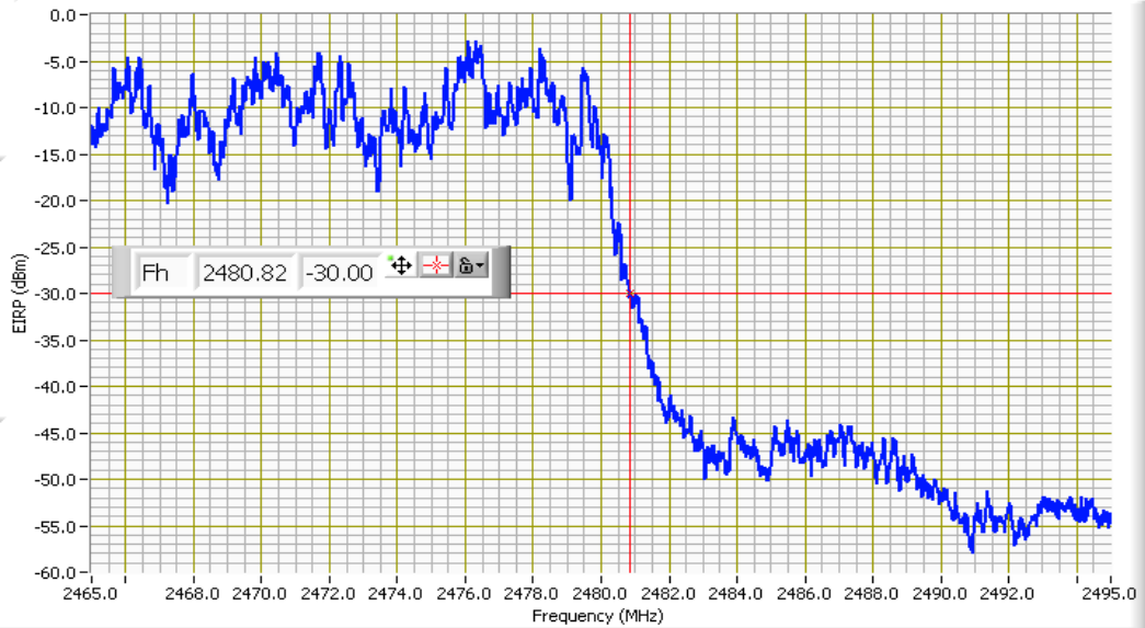
EN 300 328 Frequency Range at -10 °C, FH
