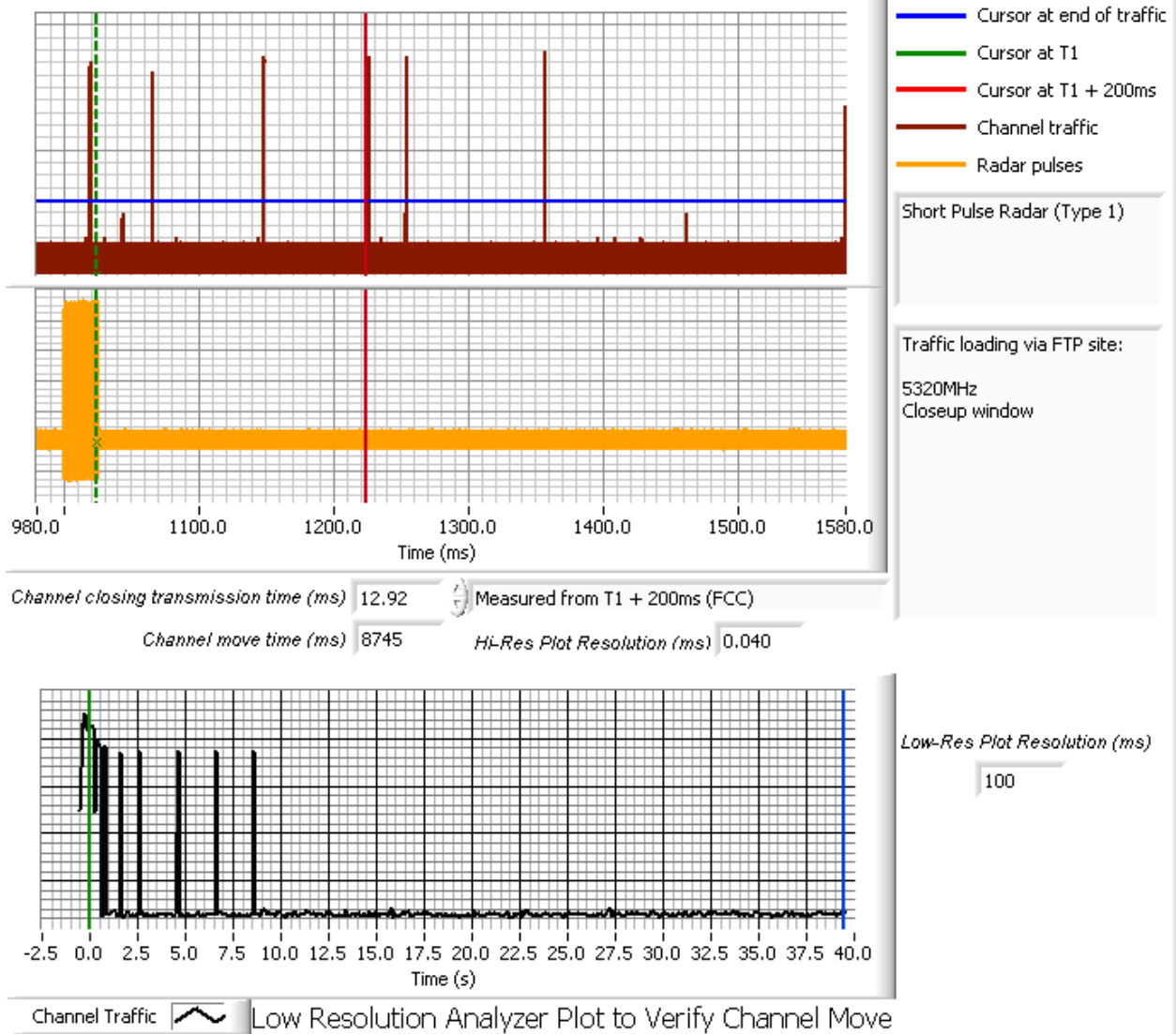
Figure 4 Close-Up of Transmissions Occurring More Than 200ms After The End of Radar 5320MHz
